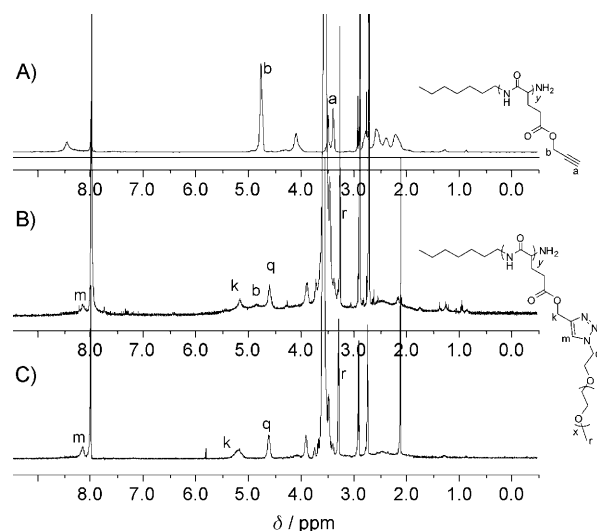
Figure 2. ^1\text{H} NMR spectrum of (A) PPLG in [\text{D}_7]\text{DMF} . (B) PPLG-g-PEG (MW = 1000 \text{g mol}^{-1} ) with a feed ratio PPLG/PEG- \text{N}_3 of 1:0.5 in [\text{D}_7]\text{DMF} . (C) PPLG-g-PEG (MW = 1000 \text{g mol}^{-1} ) with a feed ratio PPLG/PEG- \text{N}_3 of 1:2 in [\text{D}_7]\text{DMF} .
