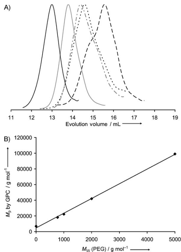
Figure 3. A) DMF GPC traces for PPLG-g-PEG. --- PPLG, ---- PPLG-g-PEG 750, - - - PPLG-g-PEG 1000, — PPLG-g-PEG 2000, — PPLG-g-PEG 5000. B) PPLG-g-PEG molecular weight as a function of grafted PEG-N 3 molecular weight.
